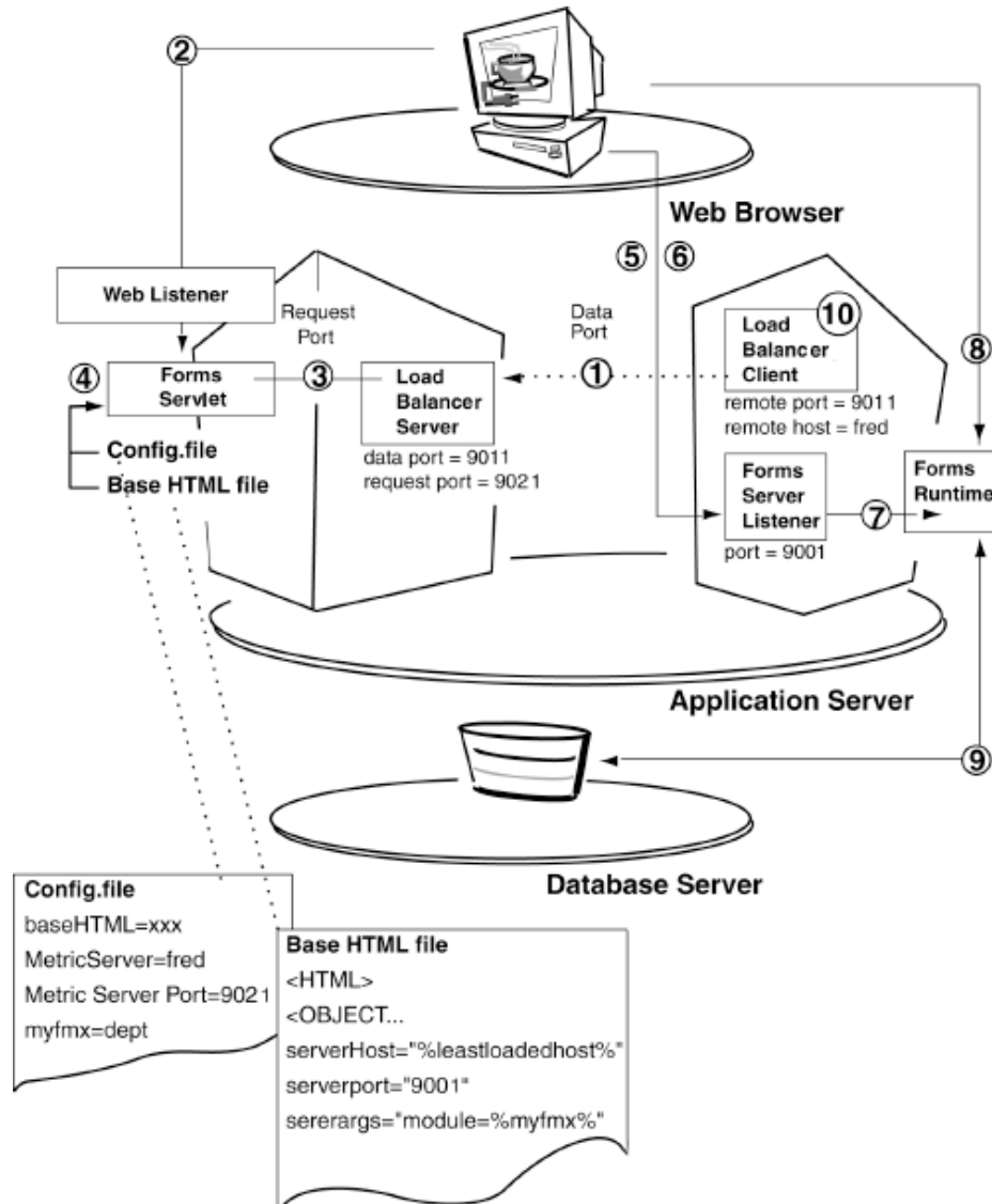
Figure 12-1 Form Services load balancing
